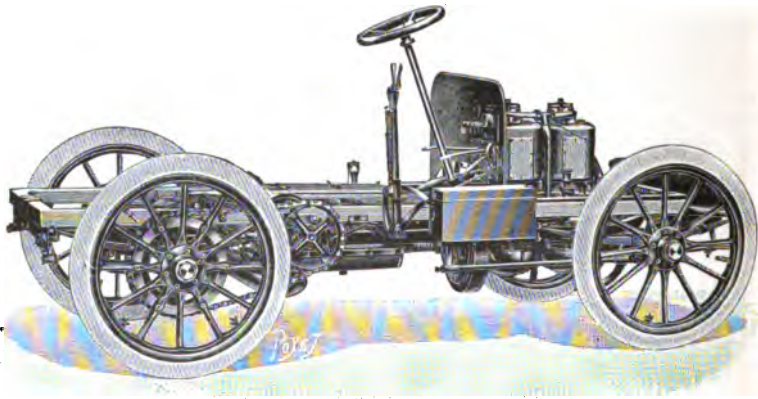
FIG. 377.—Running Gear of the Charron carriage; one of the newer makes of French automobiles, constructed on the general models of the Panhard-Levassor. The completed carriage is shown on page 330.
